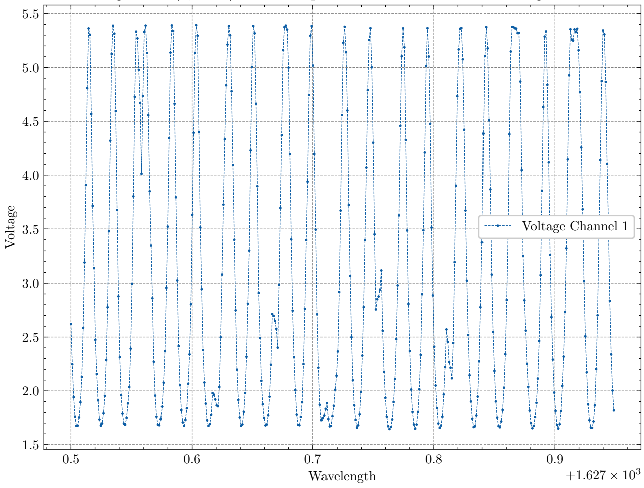
Voltage Data (0, 9999) LUT Interpolated with 3 Intermediate Integer Values
